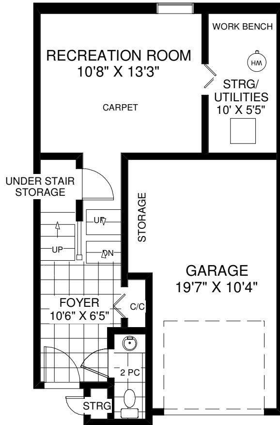
ENTRY / LOWER FLOORS APPROXIMATELY 410 SQ FT
