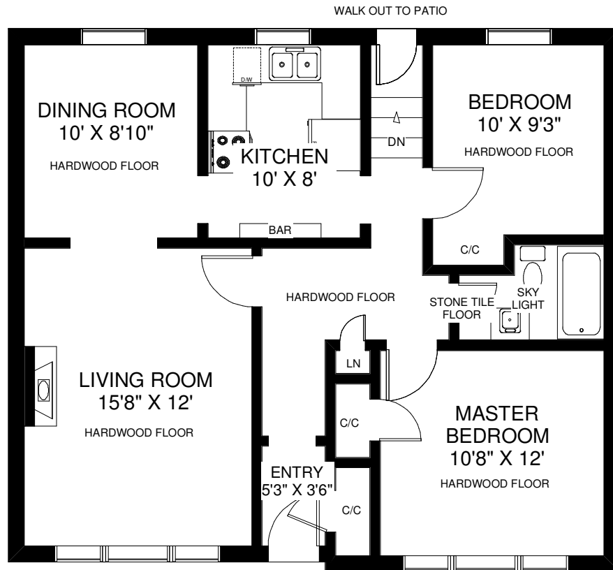
MAIN FLOOR APPROXIMATELY 900 SQ FT
