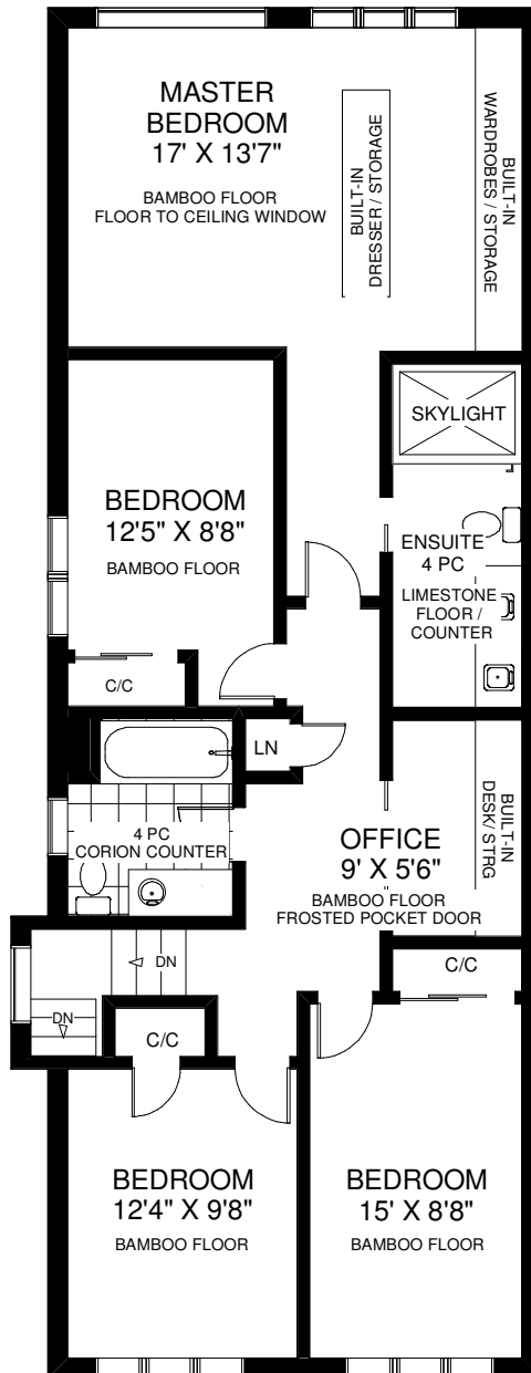
SECOND FLOOR APPROXIMATELY 1,230 SQ FT
